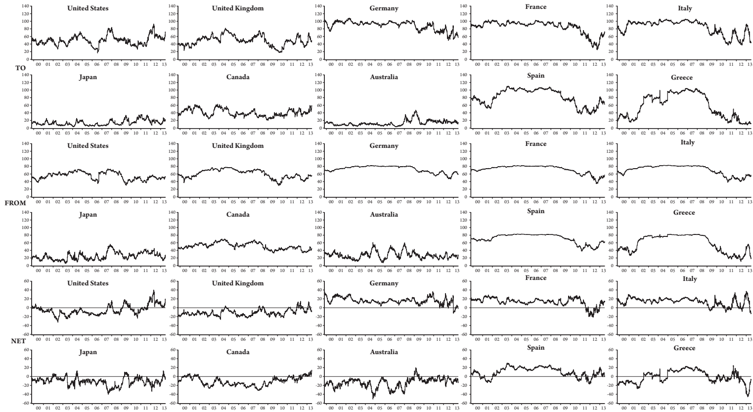
Figure 5.7 Directional bond yield volatility connectedness (200-day window).
