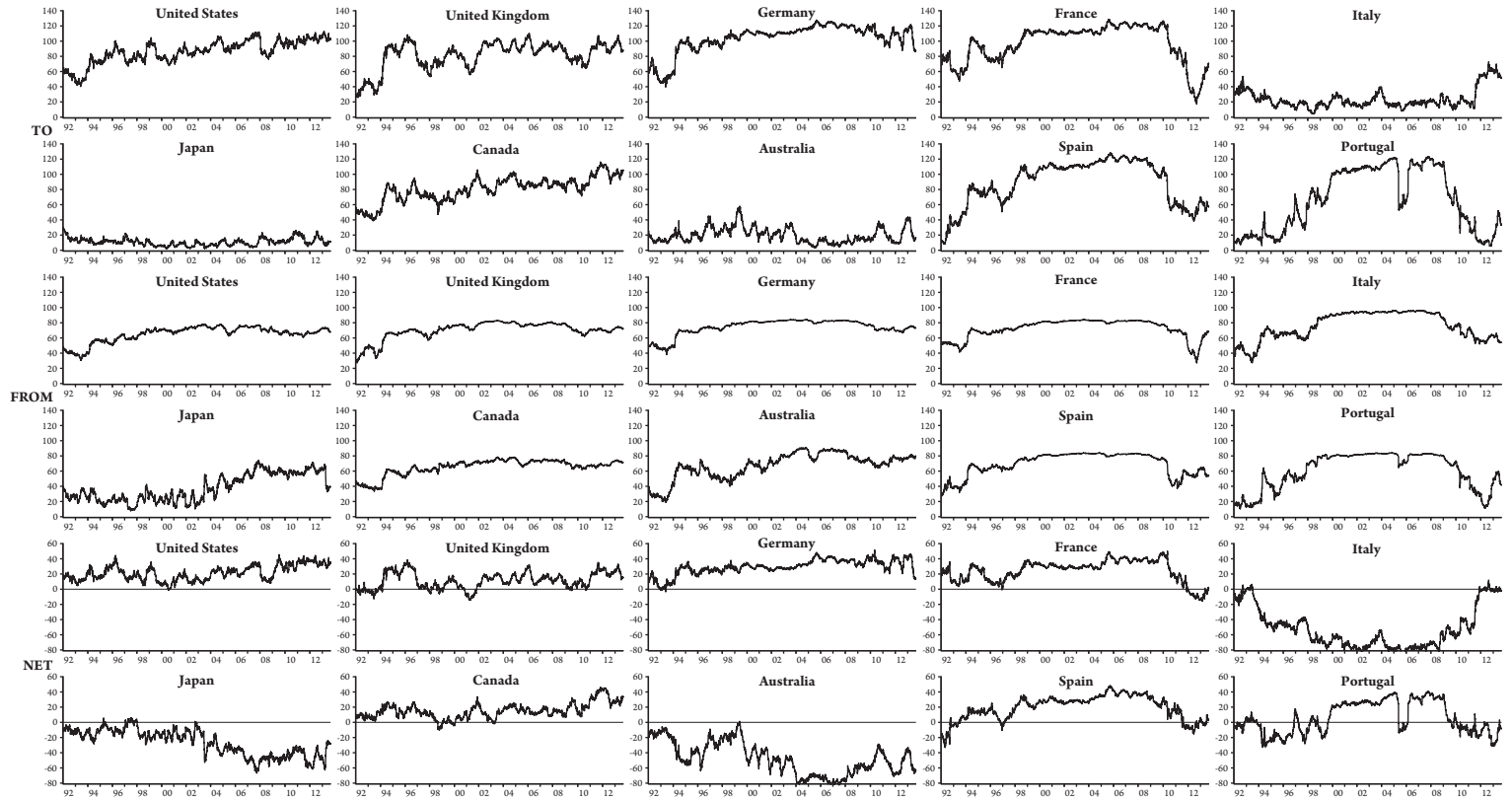
Figure 5.3 Total directional return connectedness (200-day window).
