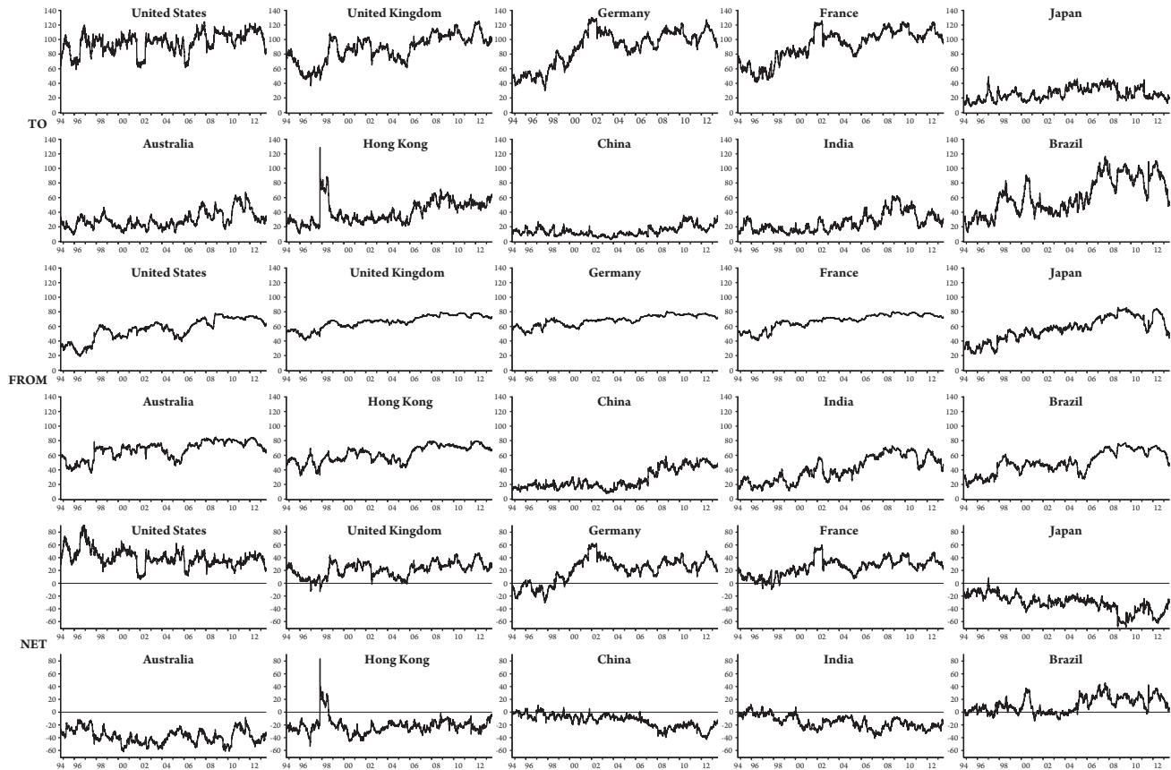
Figure 4.4 Total directional return connectedness—10 major stock markets (200-day window).
